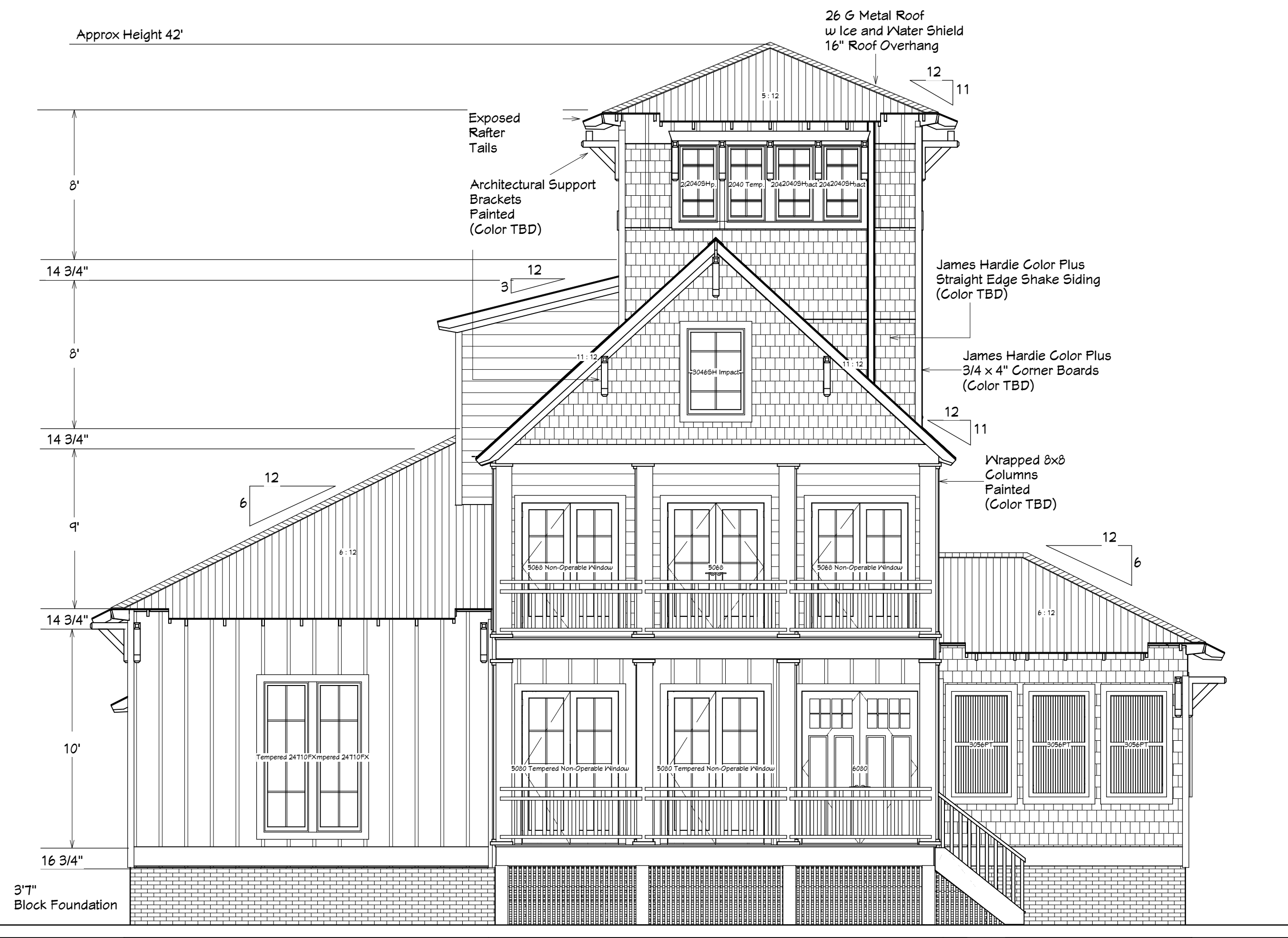
Front Elevation
