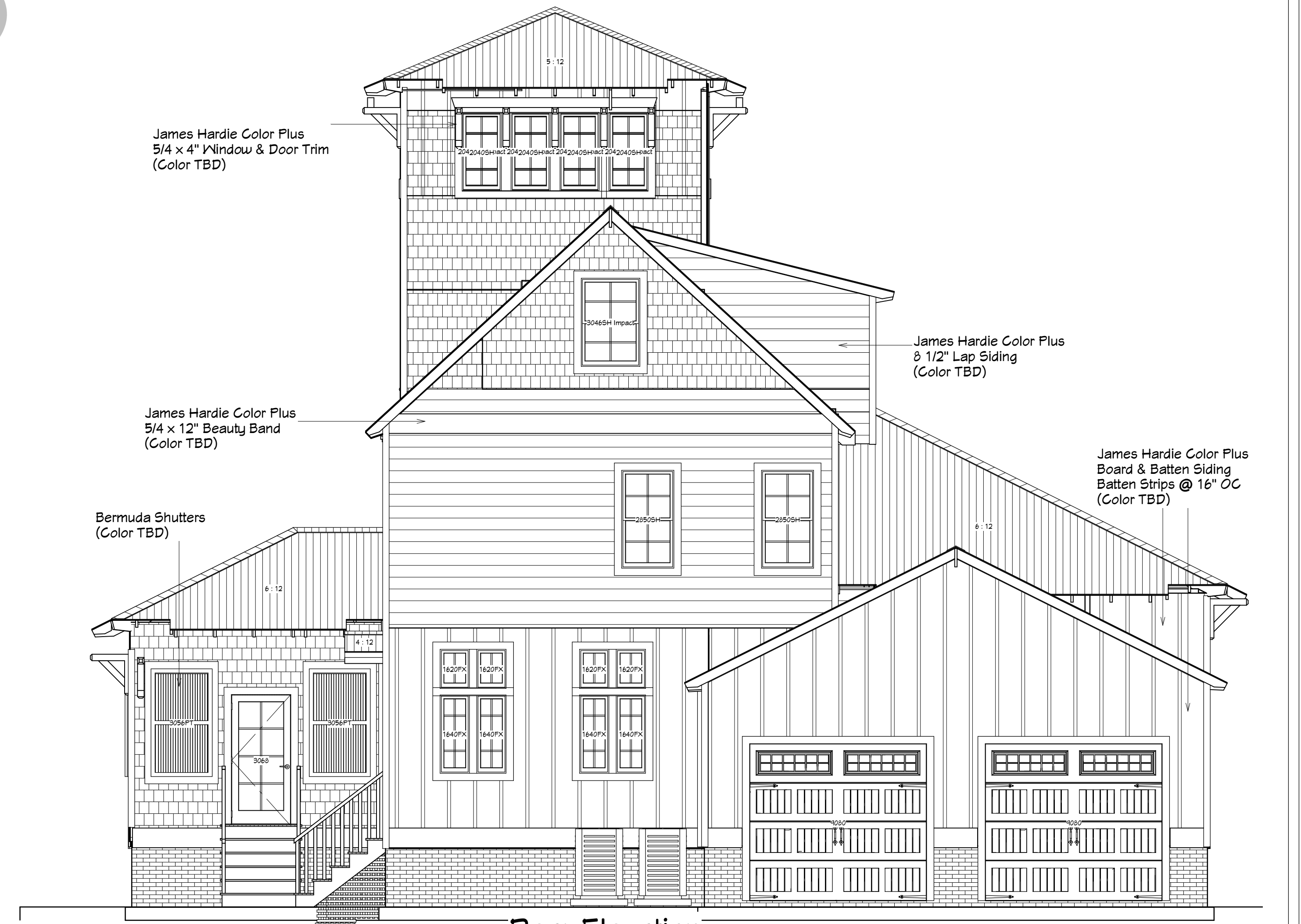
Rear Elevation
